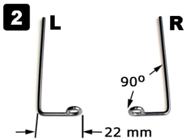
Bend mounting wires as shown.
