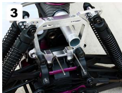
Install the mounting wires onto the lower shock tower mounting screw holes.
